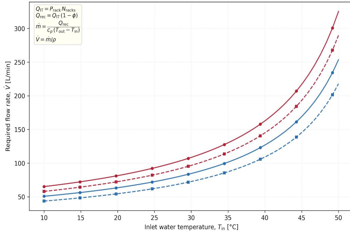
Water flow vs inlet water temperature
